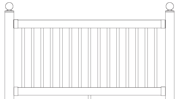
2" x 3 1/2" Top Rail Square Balusters 2" x 3 1/2" Bottom Rail
