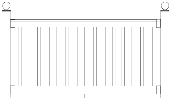
T-Shaped Top Rail Square Balusters 2" x 3 1/2" Bottom Rail
